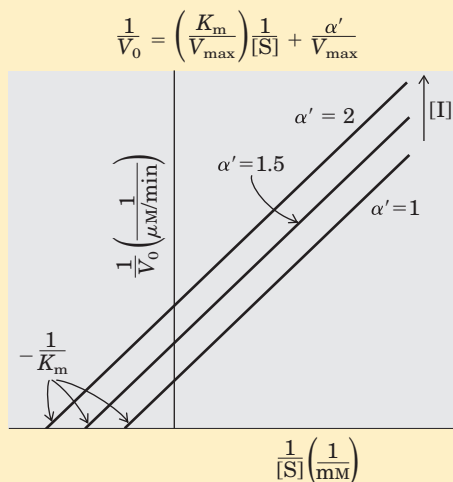
FIGURE 2 Uncompetitive inhibition.
