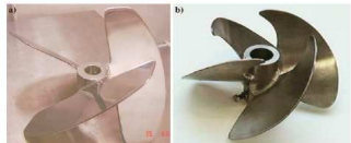
Fig. 13 (a) An ABC "elephant ear" impeller (used down-pumping); (b) Hayward Tyler up-pumping B2 hydrofoil
