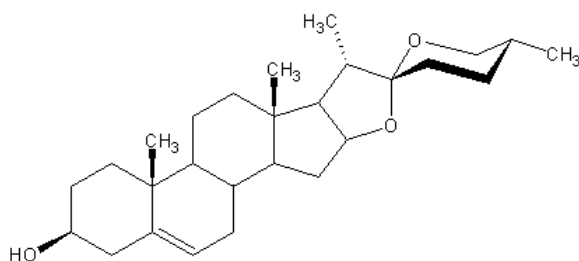
Diosgenin
